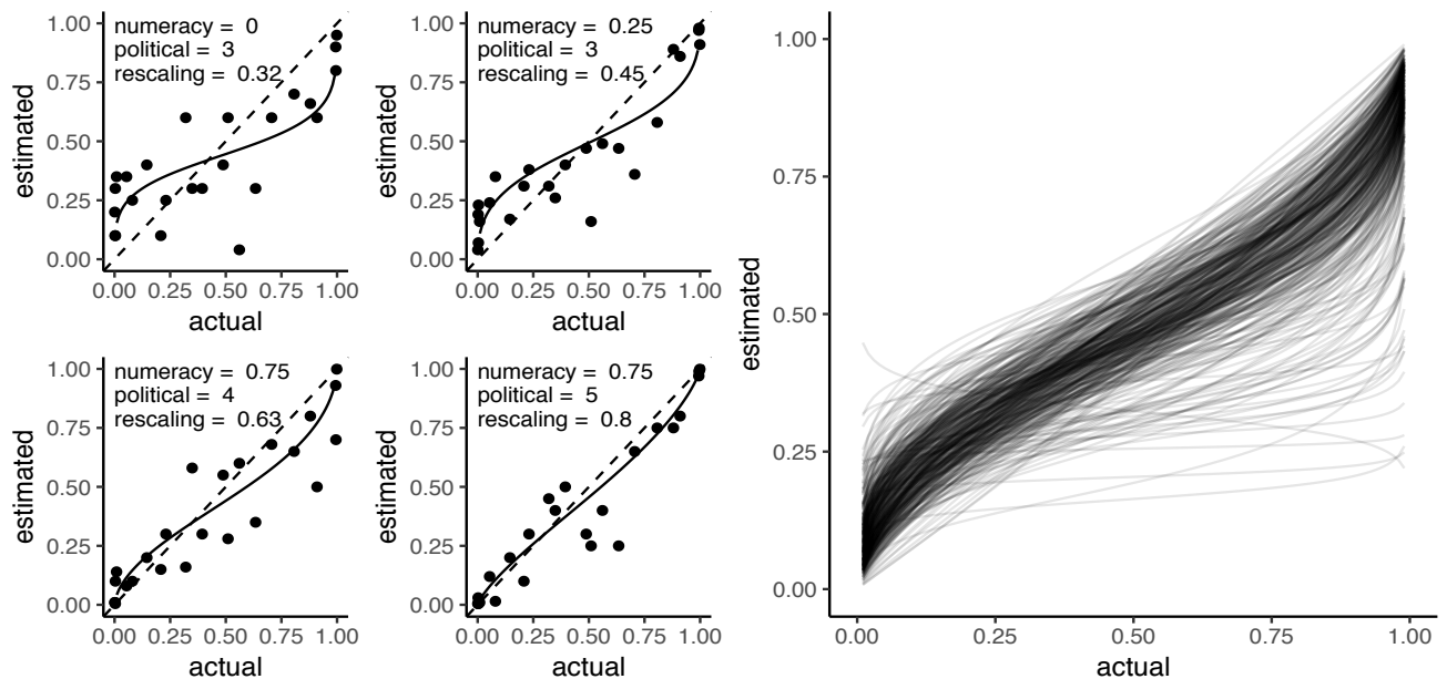
Figure 2. (Left) Sample individual estimates and model fits, illustrating how uncertainty related to rescaling. More uncertainty due to poor numeracy (worst = 0, best = 1) or poor political knowledge (worst = 0, best = 5) was associated with more rescaling (max rescaling = 0; no rescaling = 1). (Black dots = individual's estimates; black lines = predictions of rescaling model, assuming perfect underlying perceptions; dashed lines = predictions if estimates were direct reflections of underlying perceptions (i.e., without rescaling). (Right) Superimposed model fits for all participants ( N = 400 ), revealing the systematic pattern of over- and underestimation that is typical of proportion estimation under uncertainty.
